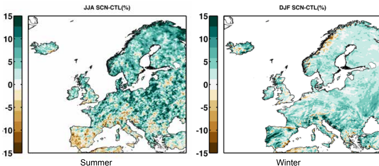
Figure 11. The increase in heavy precipitation events with a return period of 20 years.
